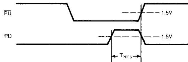
FIGURE 3: PUMPUP TO PUMPDOWN TIMING
