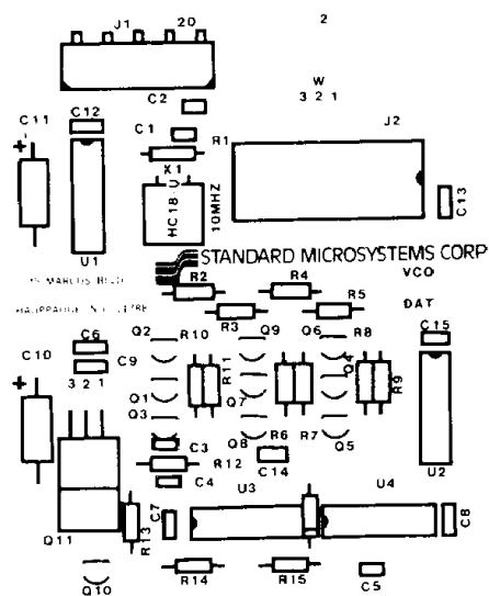
SILK SCREEN
