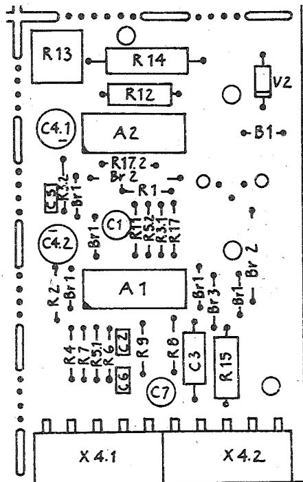
BLP RPS 5 LP - TYP 062 - 9290 1.62.519290.6/09 G
