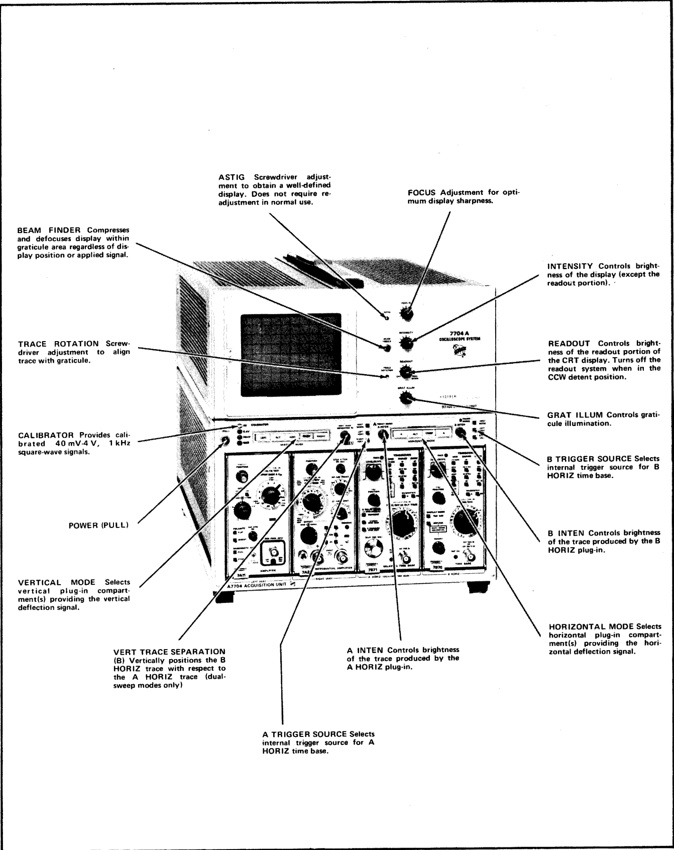
Fig. 1-2A. Front-panel controls and connectors.
