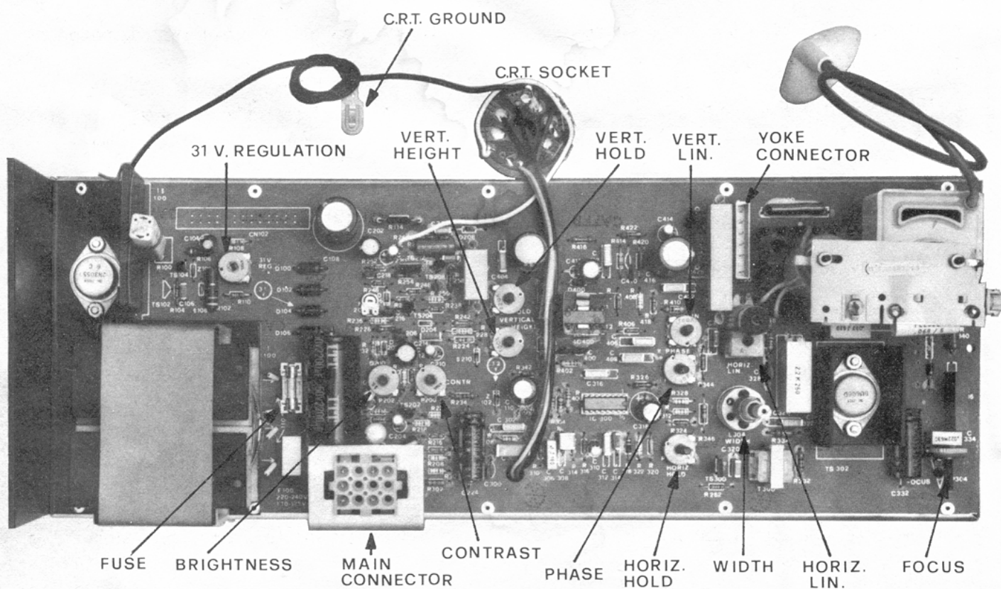
VG 978 - CHASSIS - TOP VIEW
